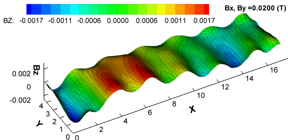
Figure 6. B_z of the busbar design in Figure 5 also presented in Figure 2 of [4].
